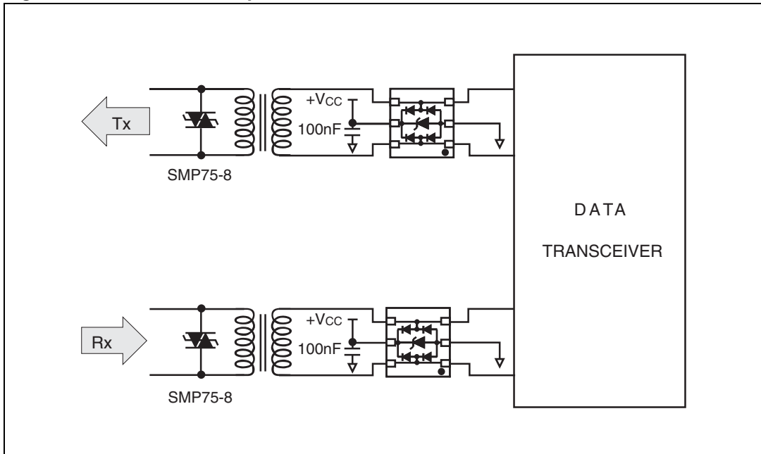
Figure 13. T1/E1/Ethernet protection
